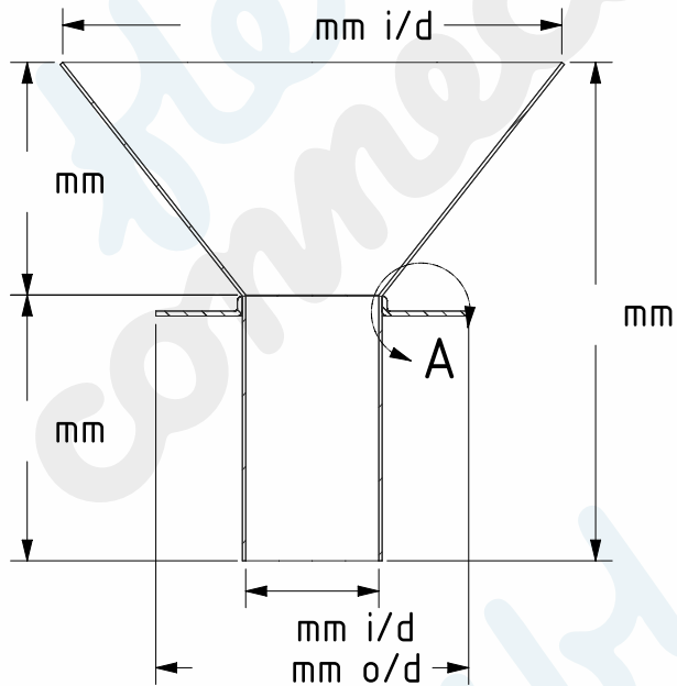
SECTION X-X
